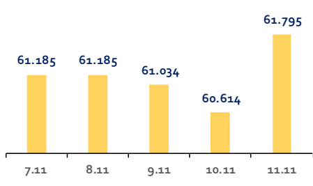
Hindistan-Sensex
